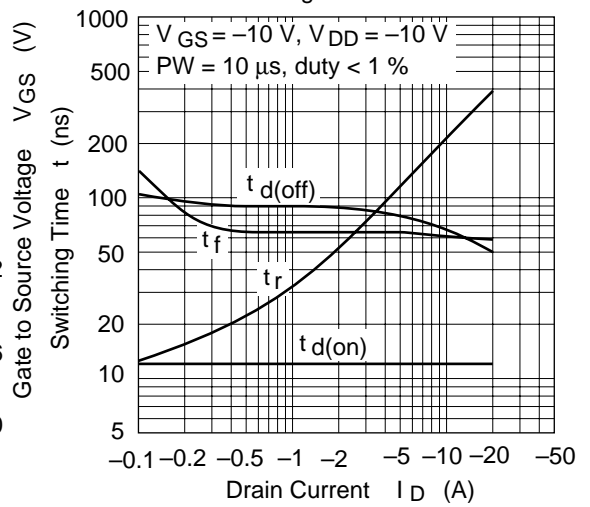
Switching Characteristics
