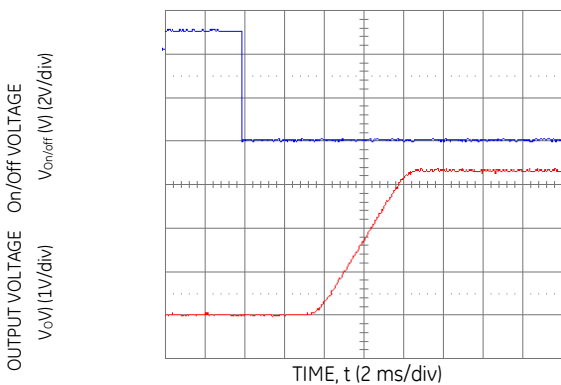
Figure 15. Typical Start-Up Using Remote On/Off with Low-ESR external capacitors ( 7 \times 150\ \mu\text{F} Polymer) ( V_{in} = 5\text{Vdc} , V_o = 3.3\text{Vdc} , I_o = 5.0\text{A} , C_o = 1050\ \mu\text{F} ).
