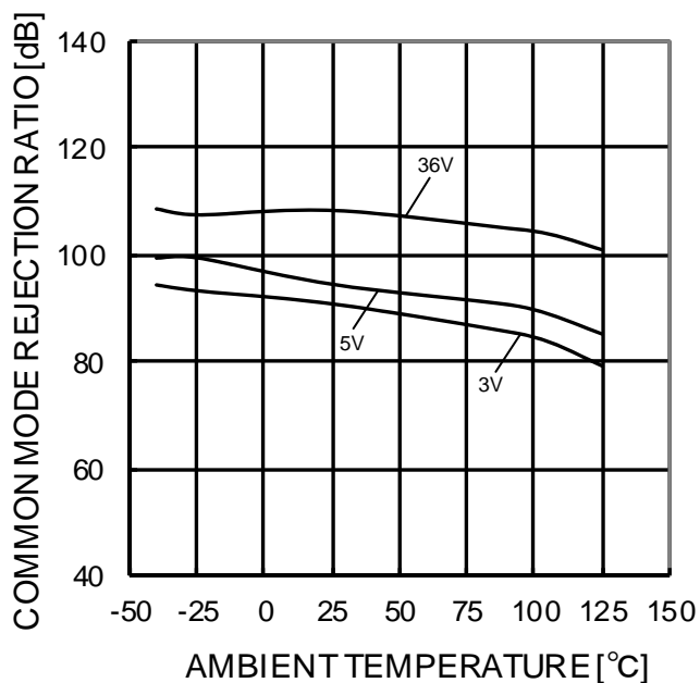
Figure 72. 同相信号除去比－温度特性
