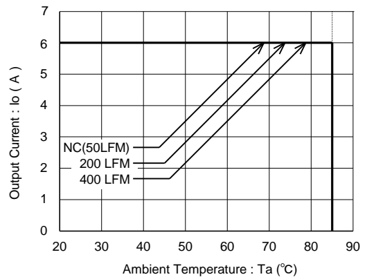
図 14 BST04M-0.7S06PDM (Vin=5.0V, Vo=0.7525V)
