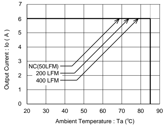
図 12 BST04M-0.7S06PDM (Vin=5.0V, Vo=3.3V)
