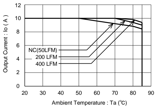
☒ 16 BST04M-0.7S10PDM ( V_{in}=5.0V , V_o=1.8V )
