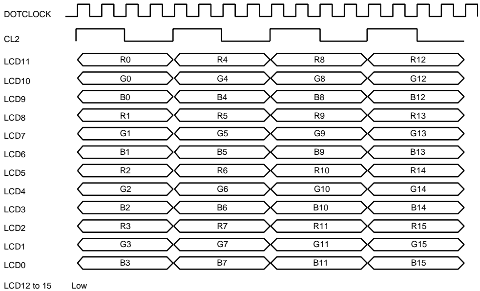
Figure 25.12 Clock and LCD Data Signal Example
