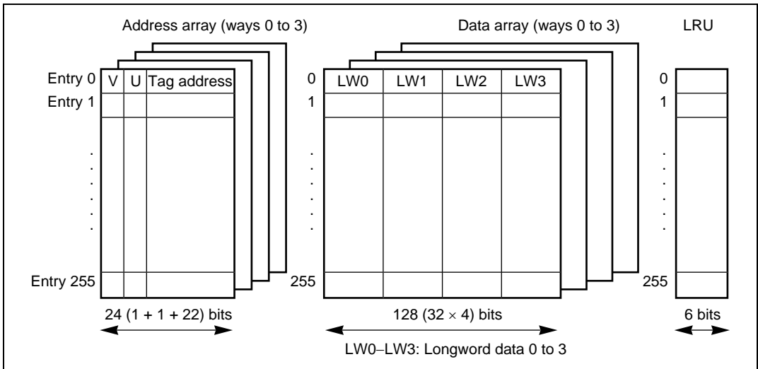
Figure 5.1 Cache Structure
