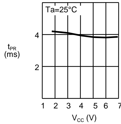
2.2 Program time t_{PR} – Power supply voltage V_{CC}
