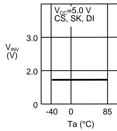
1.26 Input voltage V_{IN}(V_{IL}, V_{IH}) – Ambient temperature T_a
