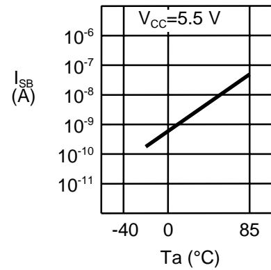
1.10 Standby current consumption I_{SB} – Ambient temperature T_a
