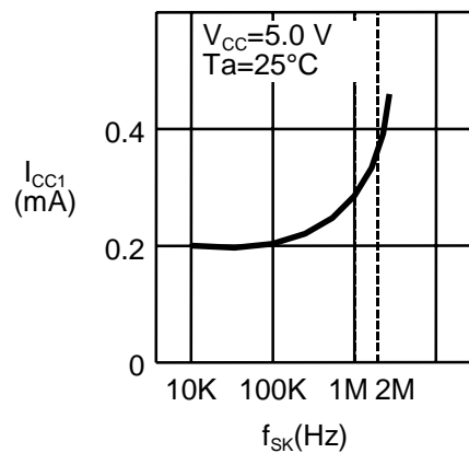
1.6 Current consumption (READ) I_{CC1} – Clock frequency f_{SK}
