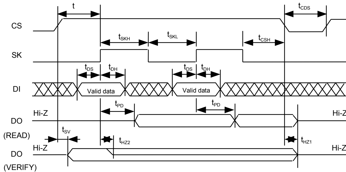
Figure 3 Timing Chart
