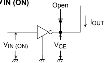
5. V_{IN} (ON)
